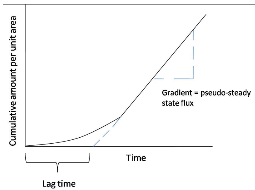
Figure 2.3 Typical permeation profile for an infinite dose application of skin membranes
