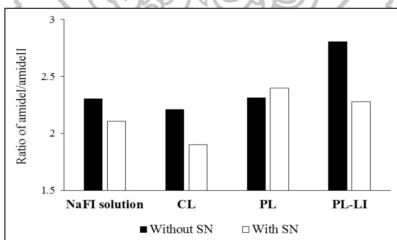
Figure 4.23 The ratio of the amide I /amide II band from FTIR spectra of the stratum corneum treated with different liposome formulations with and without SN.
