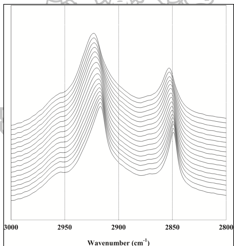
Figure 4.24 FTIR \text{CH}_2 asymmetric and symmetric spectra versus temperature of untreated stratum corneum. The temperature was in the range of 20 °C to 100 °C (top).
